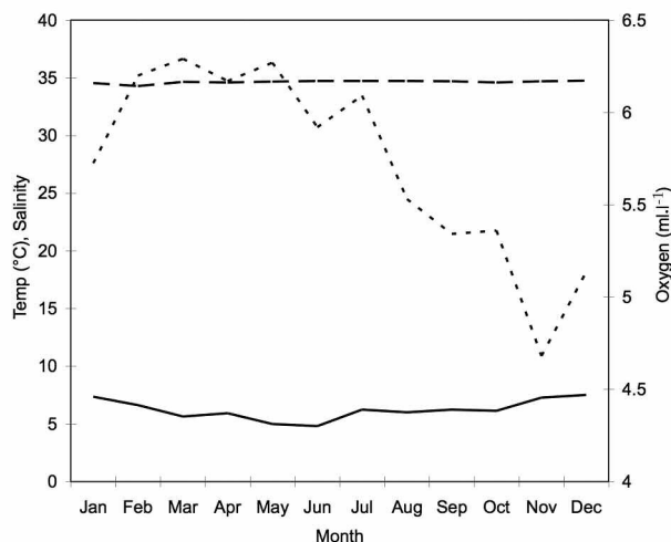
Figure 2. Monthly mean values of temperature, salinity and oxygen levels in Kosterfjorden, Sweden at 58°52,7'N; 11°05,3'E at 125 m depth. Data from Swedish Meteorological and Hydrological Institute. The solid line is temperature, the dashed line is salinity and the dotted line is oxygen.
